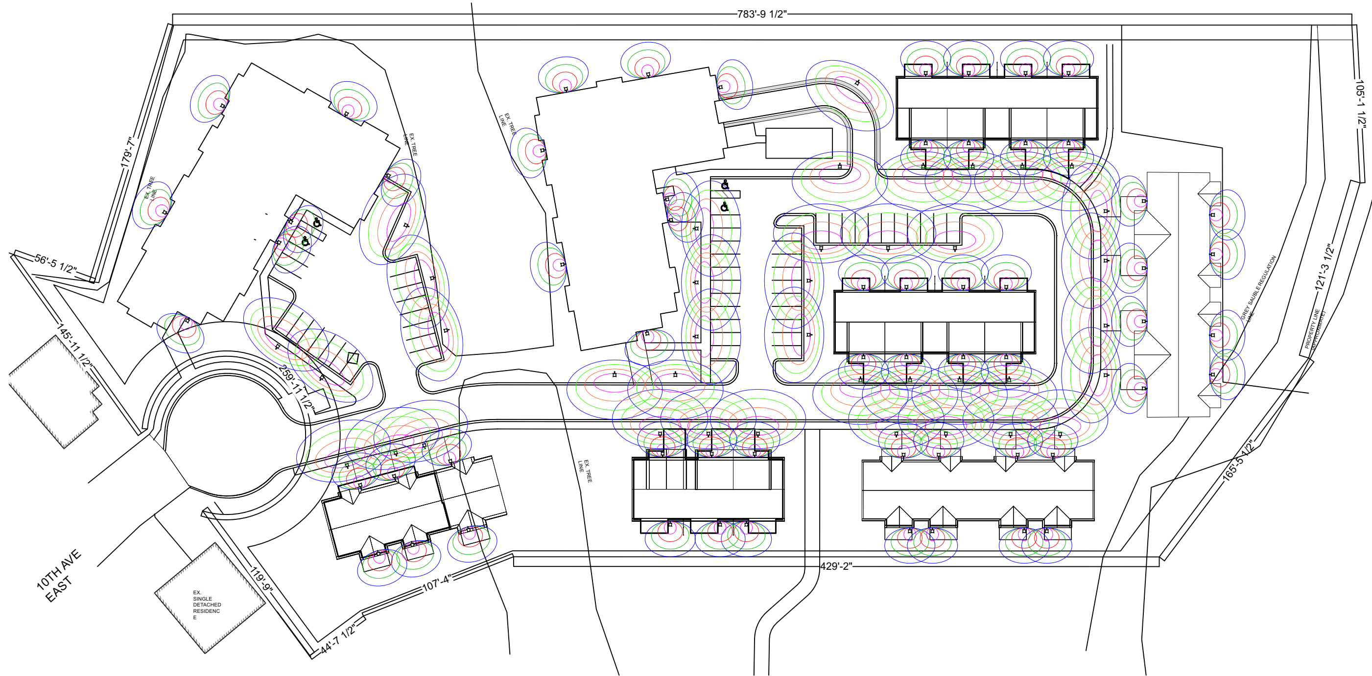
Street Lamps Scale: 1:20'-0"
